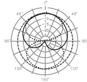
C7e Polar Response
