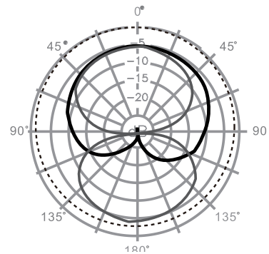
CV3 Polar Response
