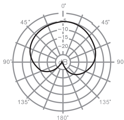
C1 Polar Response
