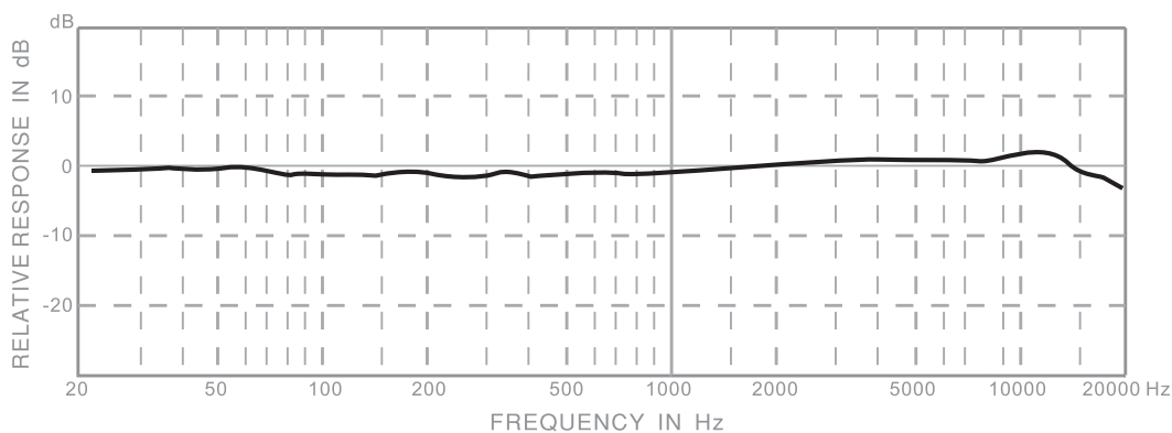
C1 Frequency Response
